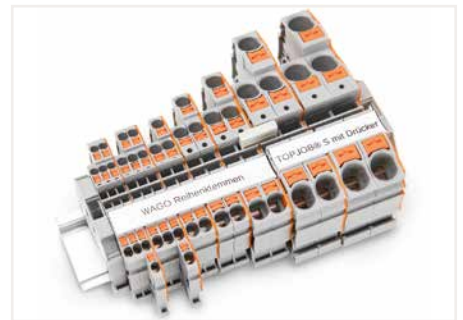
Use the same accessories for all terminal blocks.
