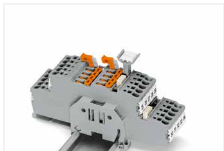
Double-deck, double-disconnect terminal blocks (2002-2951) with group marker carrier accommodated in jumper contact slot
