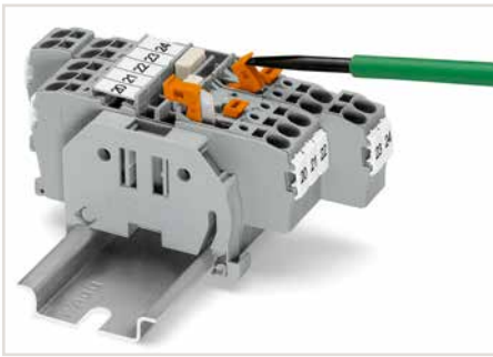
Disconnect/test terminal block with pivoting knife disconnect – Opening a knife disconnect.
