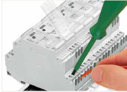
Conductor termination
