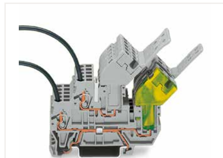
1-conductor female plug; angled Double-deck carrier terminal blocks can be commoned via 870 Series Push-In Type Jumper Bars.
